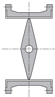
Centric
