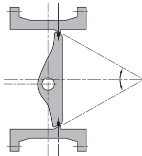
Double Eccentric
