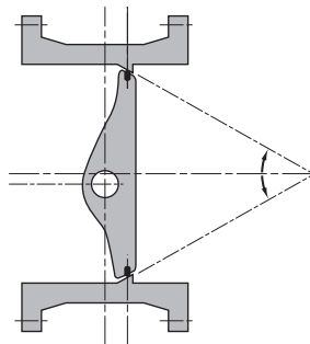
Double Eccentric
