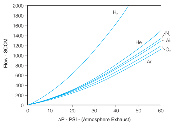
500 SCCM @ 30 psi N 2 Restrictor
