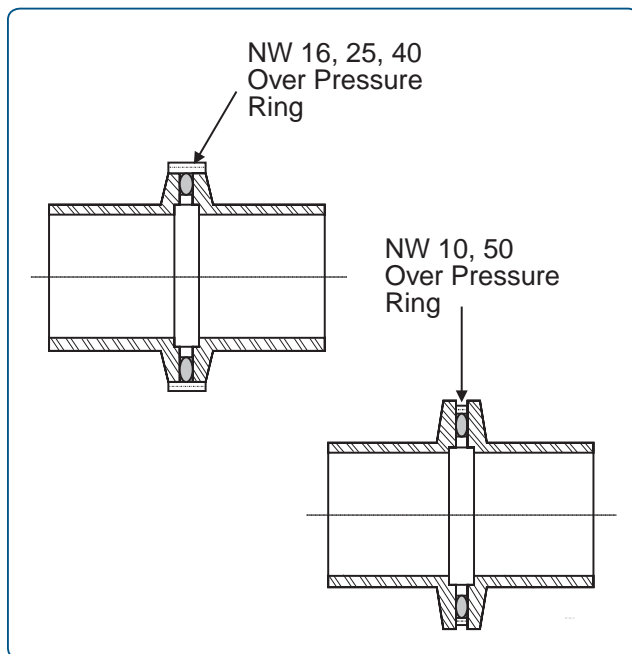
Figure 6 — Overpressure Rings
