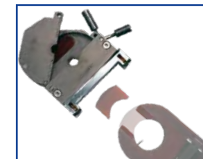
Removable Titanium clamping cassette for UHP 500-3
