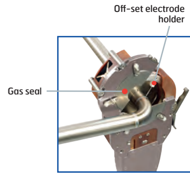
Gas seal
